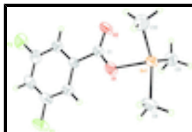
Fig. 1. ORTEP diagram of the title compound, with 50% probability displacement ellipsoids.
